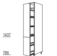
HDA*-3X 30/40 cm
