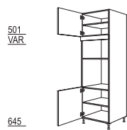
GMO-3X
