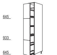
HA*-3X 30/40 cm
