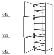
H*-3X 30/40/50/60 cm
