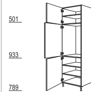
GD88-3X
